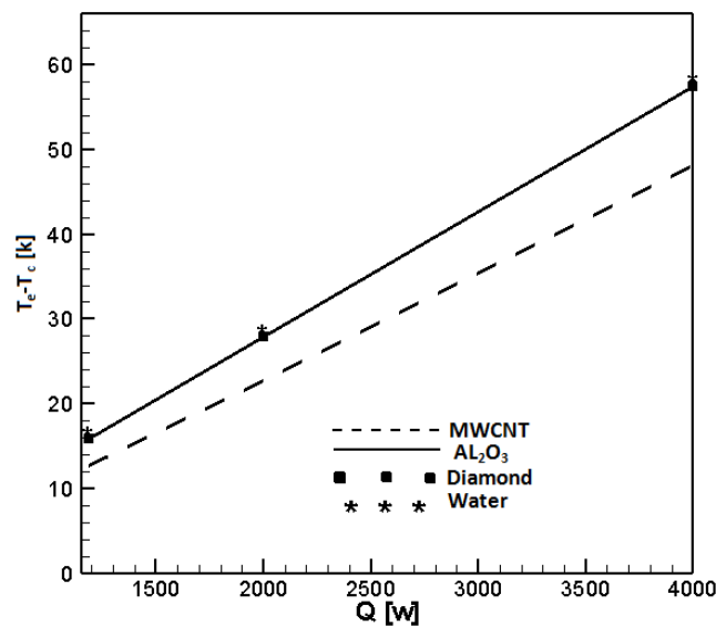
Fig. 7. The effect of heat loads on the heat pipe temperature difference
