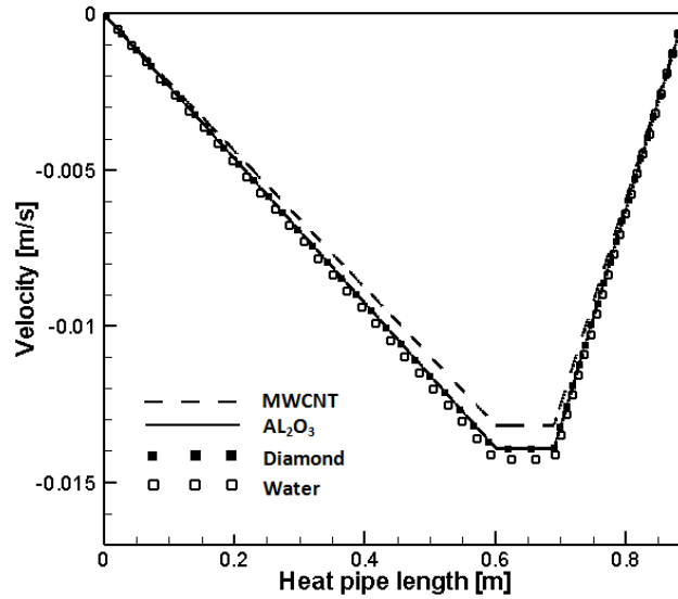
Fig. 6. The effect of different nanoparticle materials on the liquid velocity at q=1180 w
