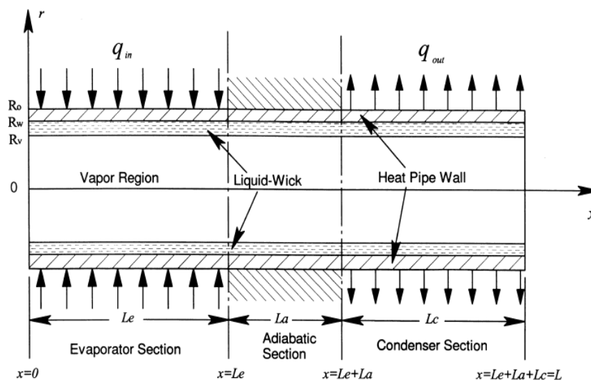
Fig. 1. Cylindrical heat pipe schematic
