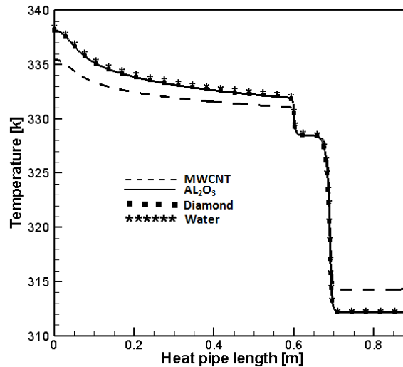
Fig. 4. Heat pipe temperature distribution; q=1180 \text{ w}
