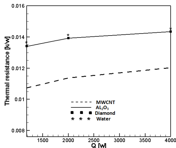
Fig. 9. The variation of thermal resistance with heat loads with different nanofluids
