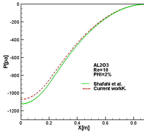
Fig. 2. Comparison of the liquid pressure distribution with analytical result by Shafahi et al. [3] at Re=10
