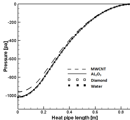
Fig. 5. The effect of different nanoparticle materials on the liquid pressure; q=1180 \text{ w}
