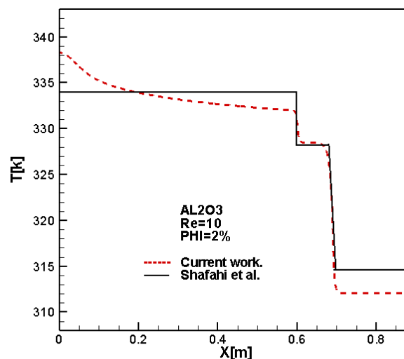
Fig. 3. Comparison of heat pipe temperature distribution with analytical results given by Shafahi [3] at Re=10
