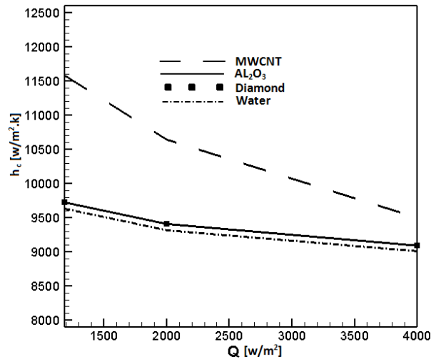
Fig. 8. The variation of heat transfer coefficient at the condenser section at different heat loads
